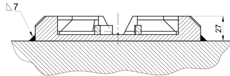
DECK OR HATCH COVER
